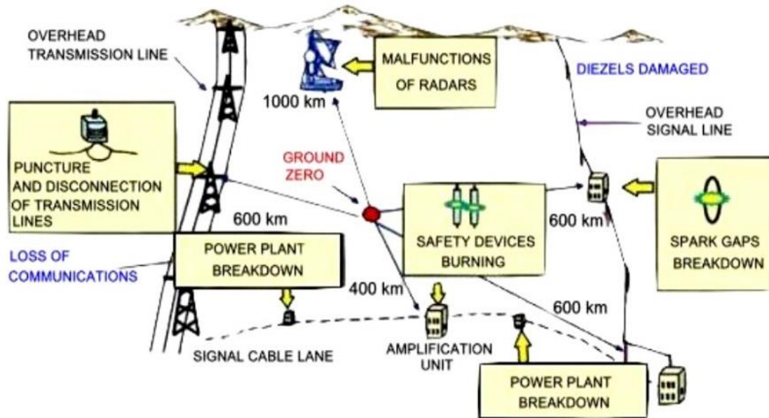
Fig. 1. Damaged electric equipment affected by HEMP during nuclear high-altitude test explosion performed under “K-3” project in Kazakhstan in 1962 (based on data published in V. M. Loborev’s report presented at EUROEM International conference in France in 1994).
